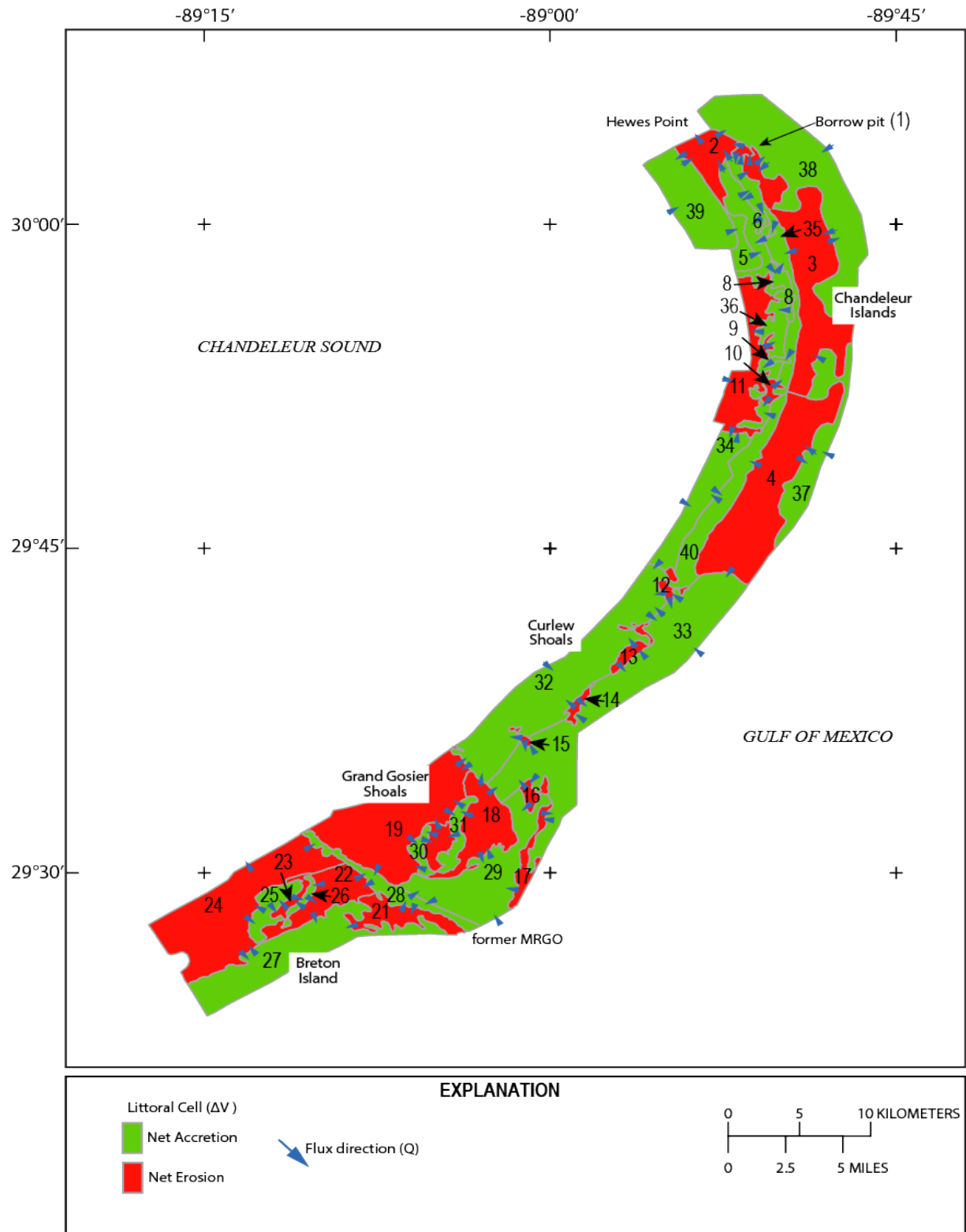
Figure 6: Littoral cells for the 2007 – 2015-time period at the Chandeleur Islands where the net volume ( \Delta V ) is positive (green) or negative (red). Blue arrows represent flux direction from (Q-source) and to (Q-sink) the cell and residual volumes are calculated to determine sediment movements and quantities.
