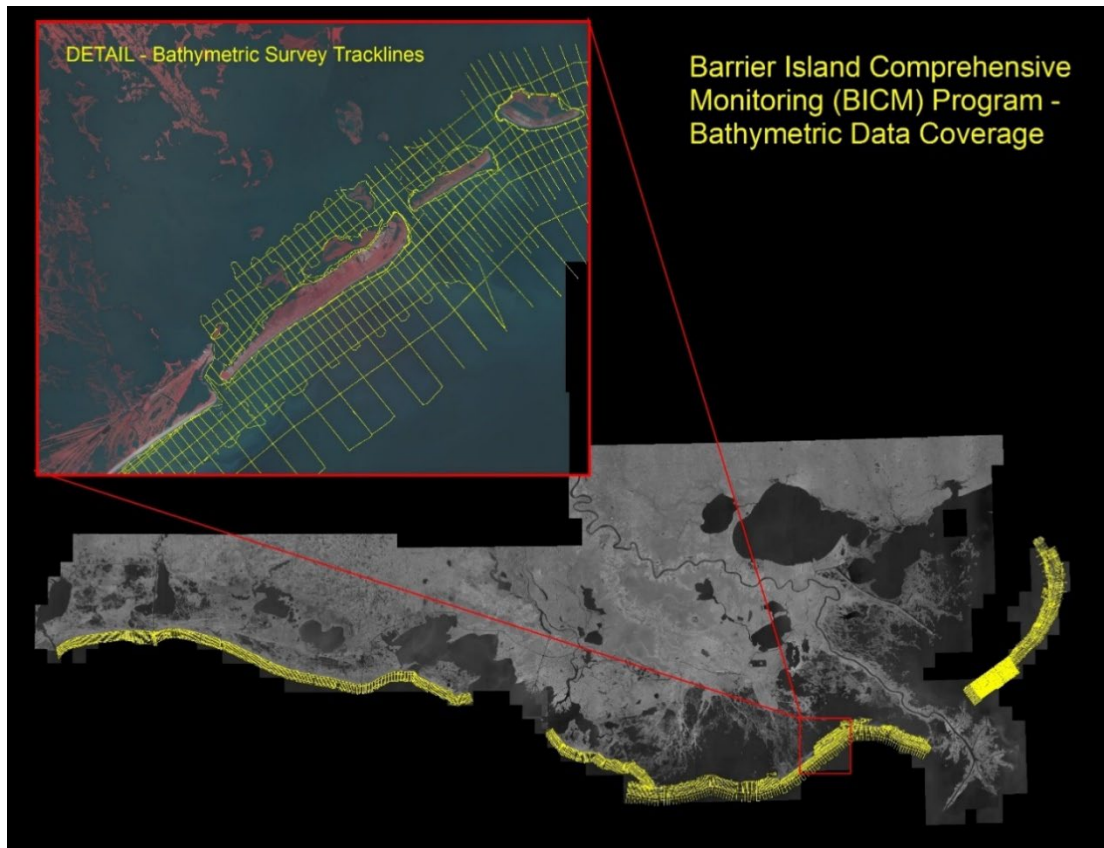
Figure 4: Bathymetric data collection coverage for the second BICM data collection cycle (2015-2019).
