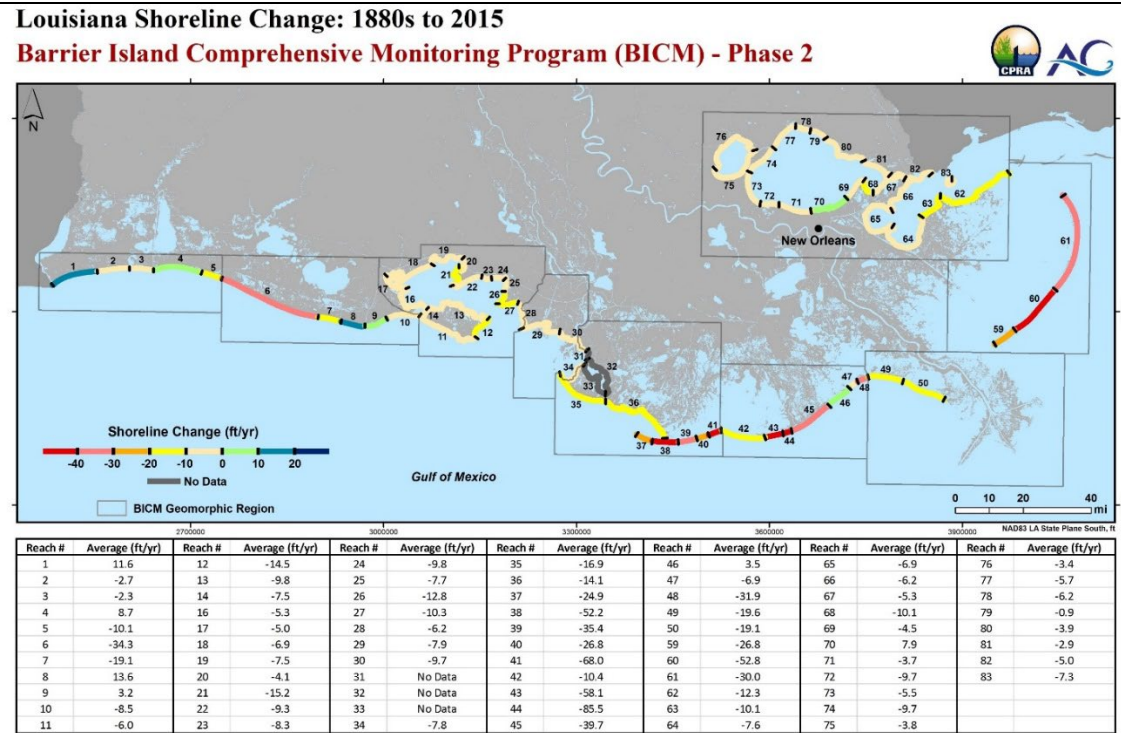
Figure 3: 1880's to 2015 average shoreline erosion rates for individual BICM shoreline reaches.
