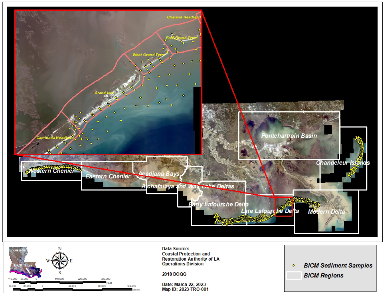
Figure 12: Location and extent of the BICM 3 surficial sediment cores.
