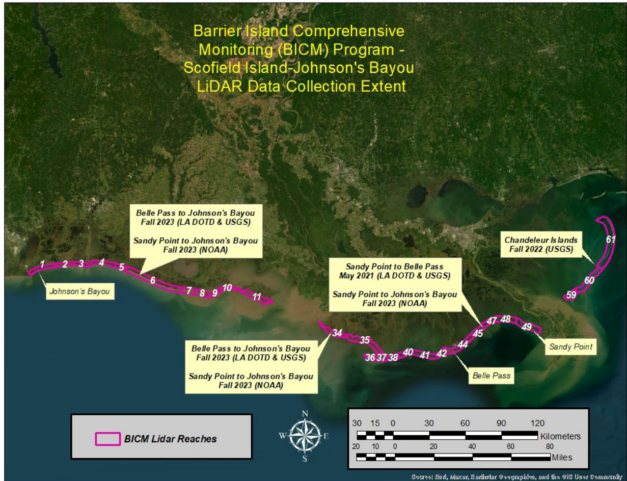
Figure 11: BICM 3 LiDAR extent and timeline.
