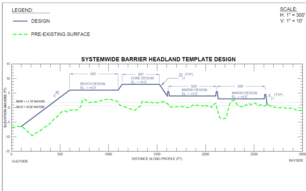
Figure 17: System-wide Barrier Headland Design Template.
