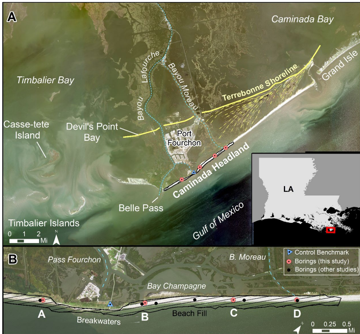
Figure 15: Site locations for sediment borings (A through D) and anchored monuments (A through C) for documenting subsurface geologic characteristics and monitoring elevation changes in response to beach restoration along the Caminada - Moreau Headland (Lafourche shoreline) in south Louisiana. The Terrebonne shoreline was formed during early Lafourche delta abandonment of the Terrebonne, Bayou Blue, and Point au Chien lobes. The beach fill polygon is the as built areal extent of the fill for Caminada Headland Restoration Project (BA-0045). CMS-BM-01 is the project control benchmark.
