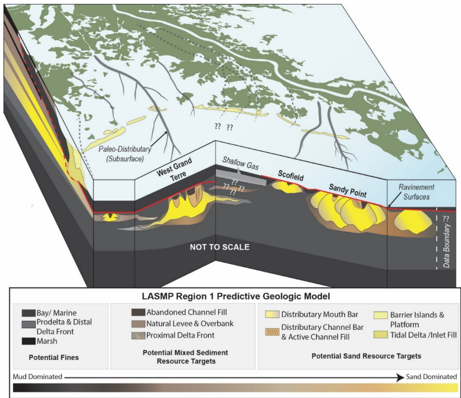
Figure 18: Predictive Geologic Models for LASMP Region 1 (Barataria-Terrebonne Basin) are 3-dimensional block diagrams and are visual communication tools to convey the components of the modern environment and subsurface geology
