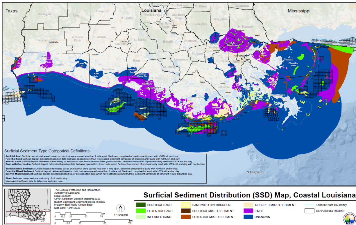
Figure 20: 2023 SSD map update showing surficial distribution of various sediment types in Coastal Louisiana.
