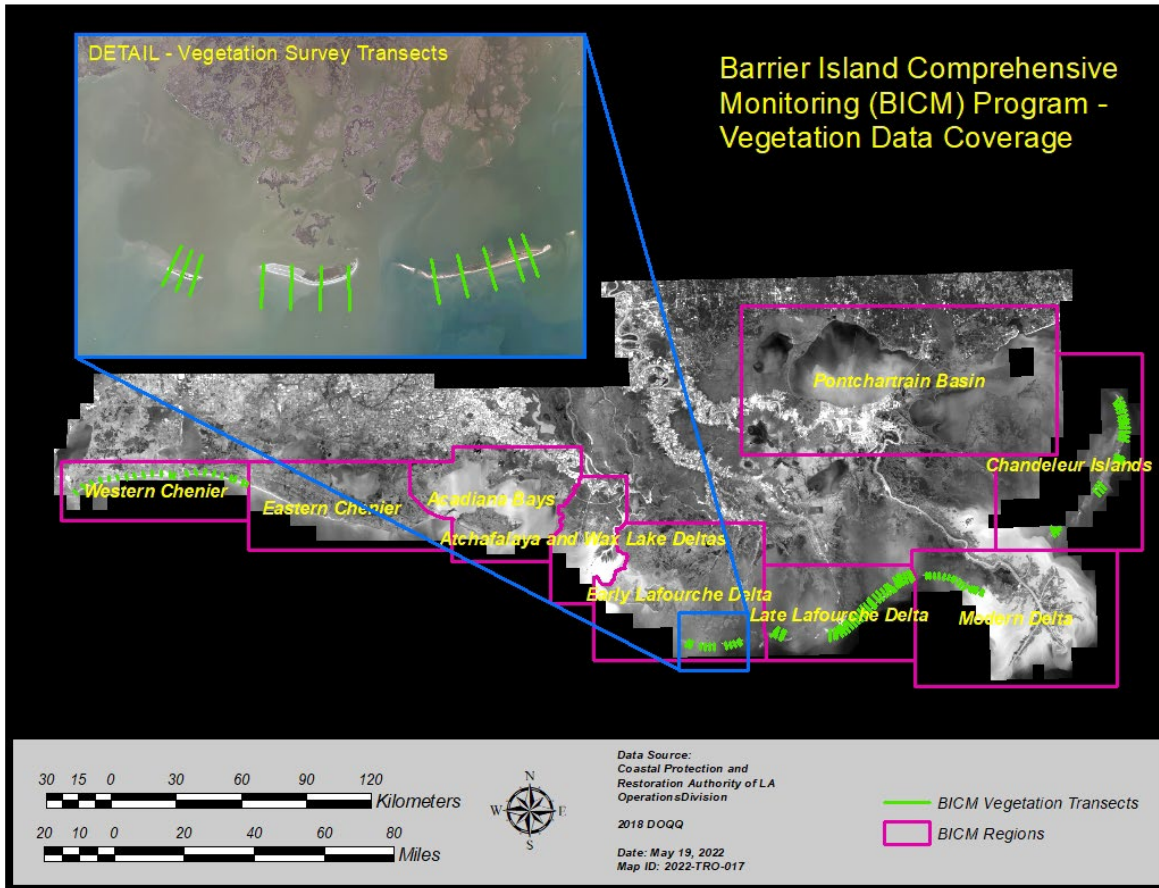
Figure 14: Location and extent of the BICM 3 vegetation transects.
