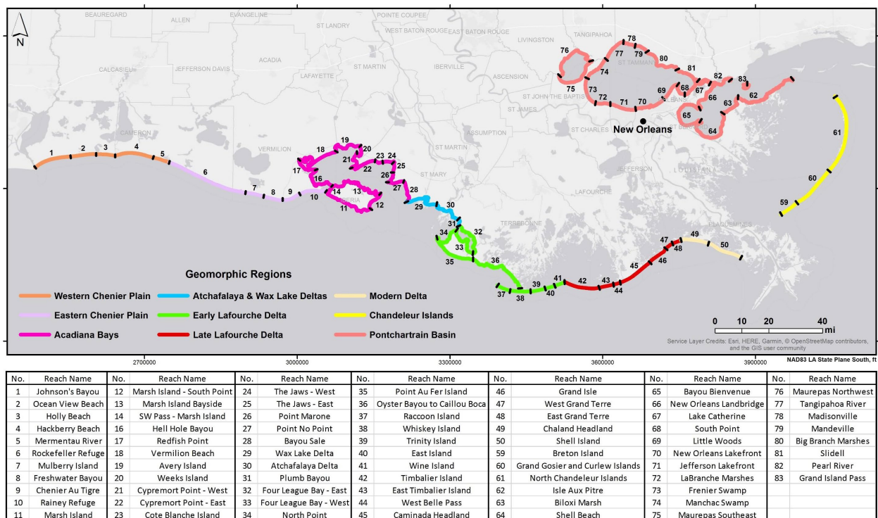
Figure 10: The BICM shoreline regions and reaches.
