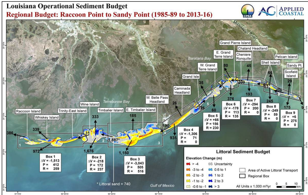
Figure 19: Macro-scale littoral sediment budget for the south Louisiana barrier shoreline, 1985-89 to 2013-16. Arrows represent net direction of sediment movement and numbers reflect magnitudes of net sediment transport in thousands of m 3 /yrs. P= Placement; R= Removal.
