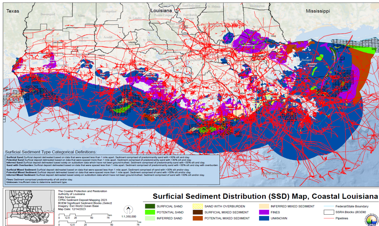
Figure 21: 2023 SSD map update showing surficial distribution of various sediment types in Coastal Louisiana overlain by oil and gas active pipelines.
