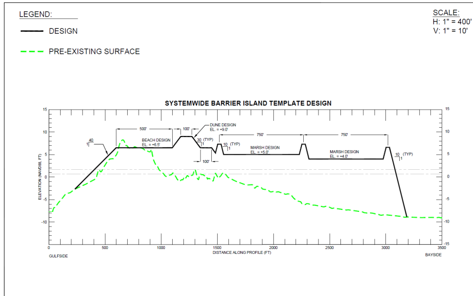
Figure 16: System-wide Barrier Island Design Template.
